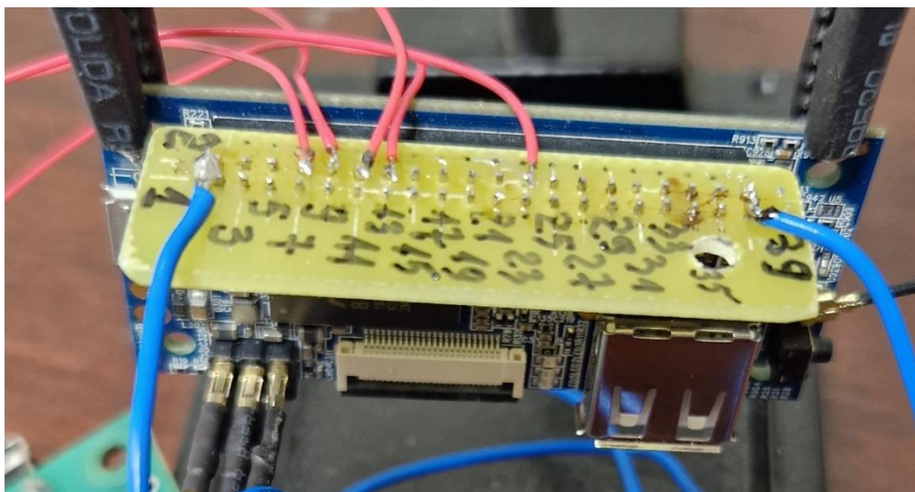
FIGURE 27 - PROTOTYPE BOARD TO CONNECT OSCILLOSCOPE PROBES BY USING 40-PINS CONNECTOR
